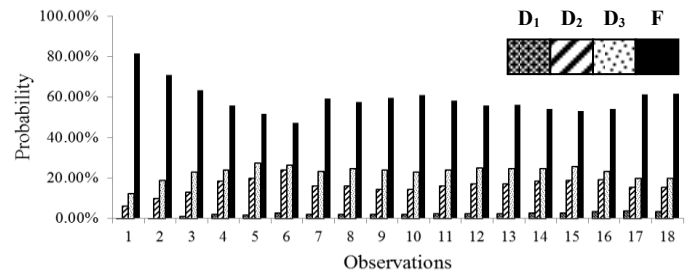
Fig. 5. Probability of the CB trip coil staying in each deterioration state.
