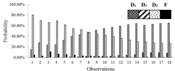
Fig. 6. Probability of the CB AB contacts staying in each deterioration state.
