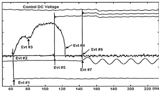
Fig. 2. Monitored coil current waveform during the CB close operation [18].
