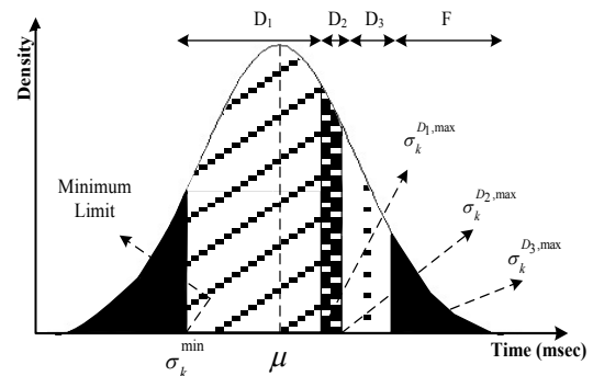
Fig. 3. Probability distribution and the bands assigned to timing parameter t_2 .
