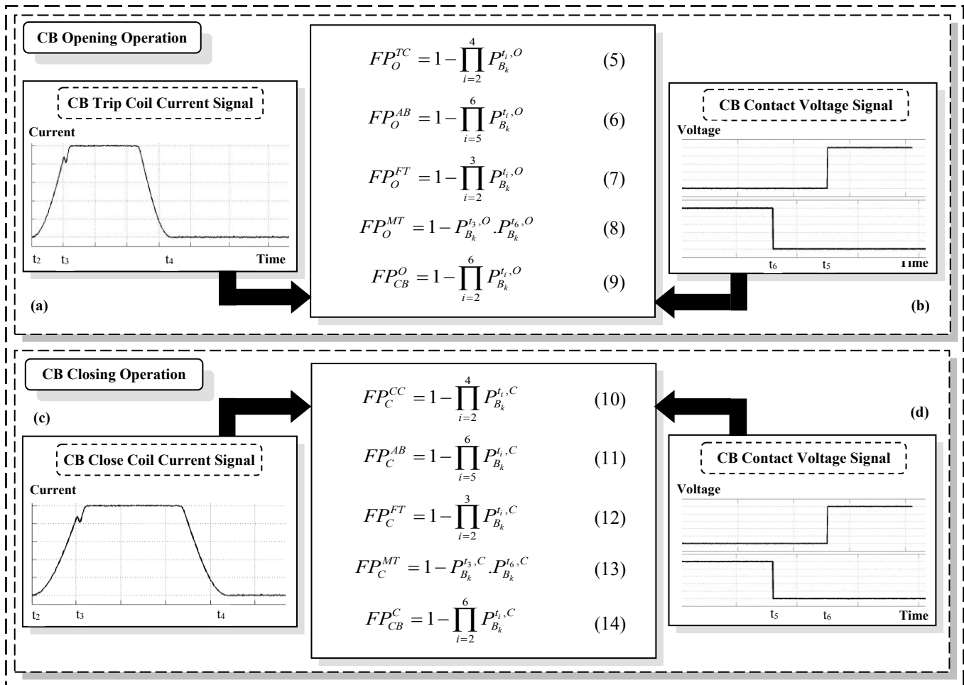
Fig. 4. General formulations for the failure probability estimation of CB subassemblies in both opening and closing operations.
