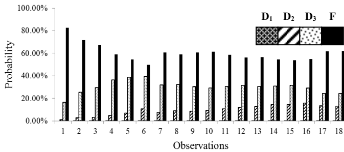
Fig. 7. Probability of the CB, as a component, in each deterioration state.
